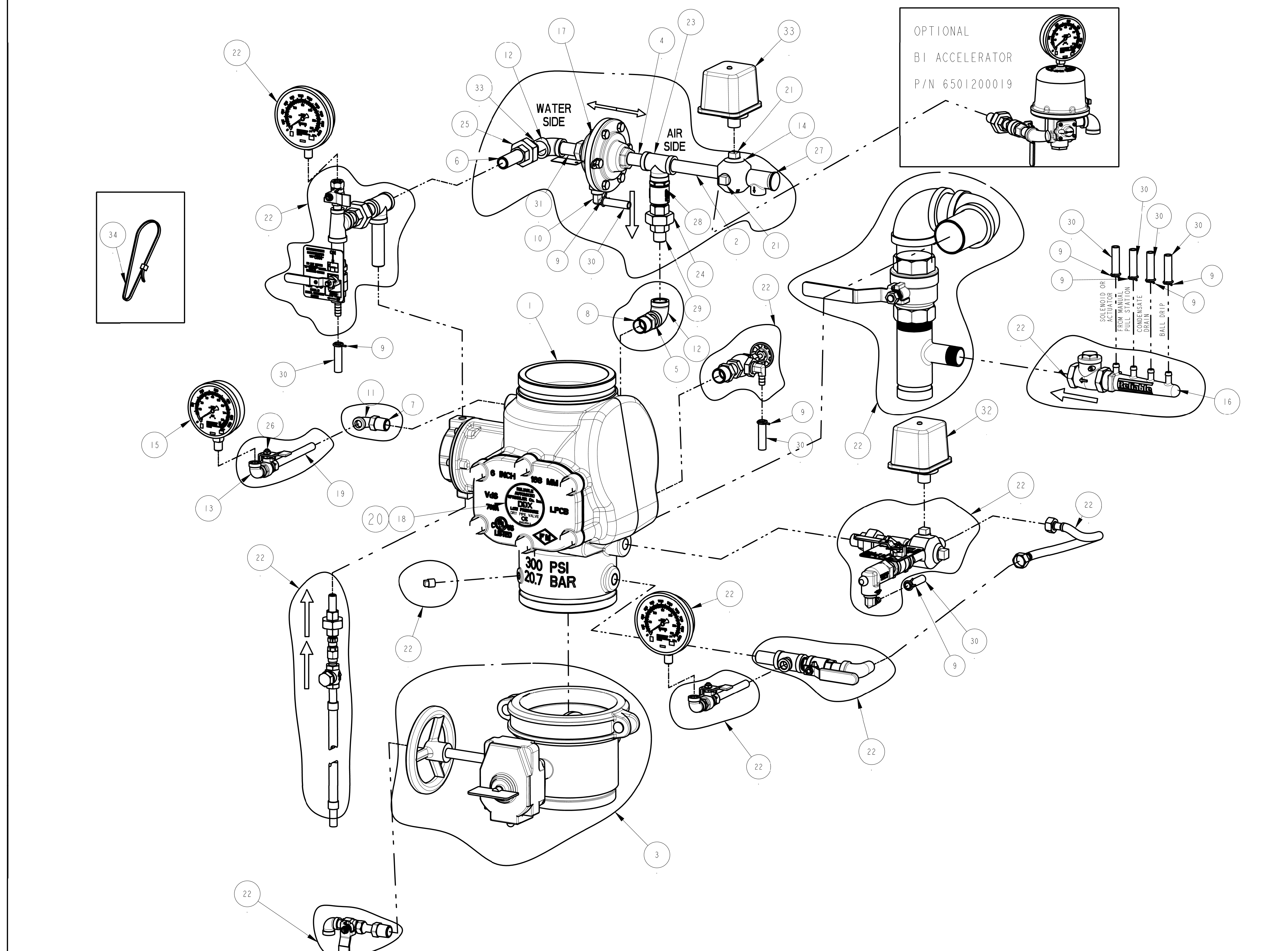
MODEL DDX 4", 6" & 8" DELUGE LOW PRESSURE DRY PIPE CA-156 P/N 8924116 REV. R
